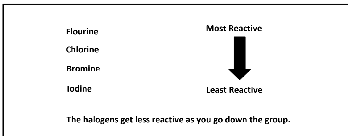
The reactivity series of halogens
