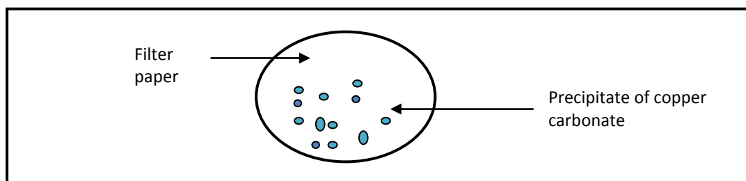
Precipitate of copper(II) carbonate after drying on a piece of filter paper.
