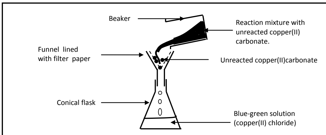
Filtration process to remove unreacted copper(II)carbonate crystals.
