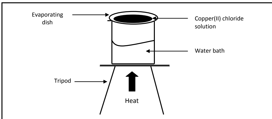
Evaporation of copper(II) chloride using water bath
